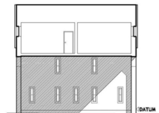
MAIN BLOCK - SECTION/WEST inner EL
